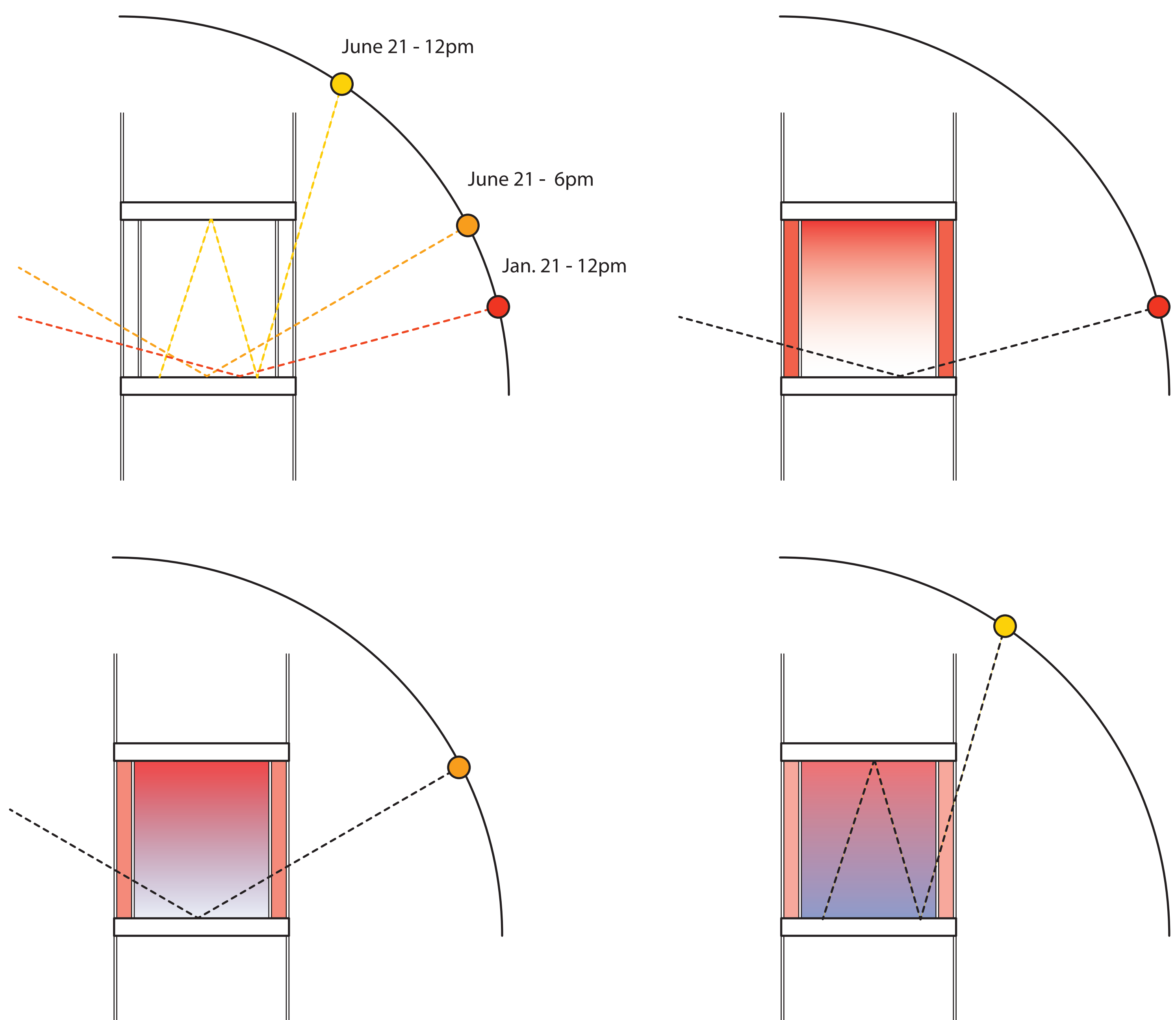
As the angle of the sun changes from summer to winter, the temperature of the double-paned, insulated reading rooms increases due to more exposure to more direct sunlight.
